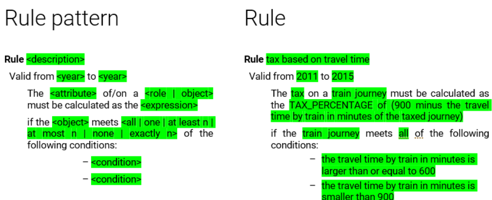
Figure 3. A RegelSpraak rule pattern (left) and substantive rule (right)
